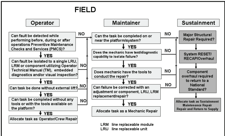
Figure E-1. Two level maintenance process flow
